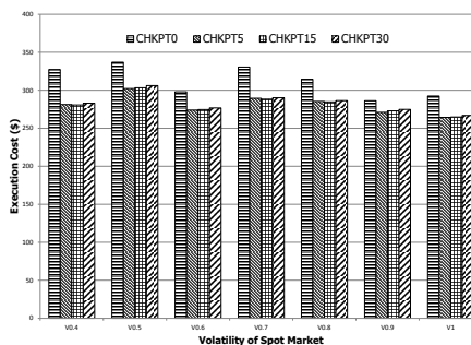
Figure 6: Effect of checkpointing on execution cost.
