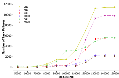
Figure 5: Mean of task failures due to bidding strategies.
