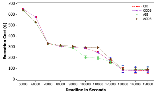
Figure 4: Mean Execution Cost of bidding strategies with varying deadline (with 95% confidence interval).
