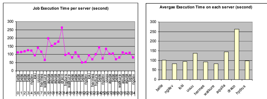
Figure 5. Job execution time statistics
