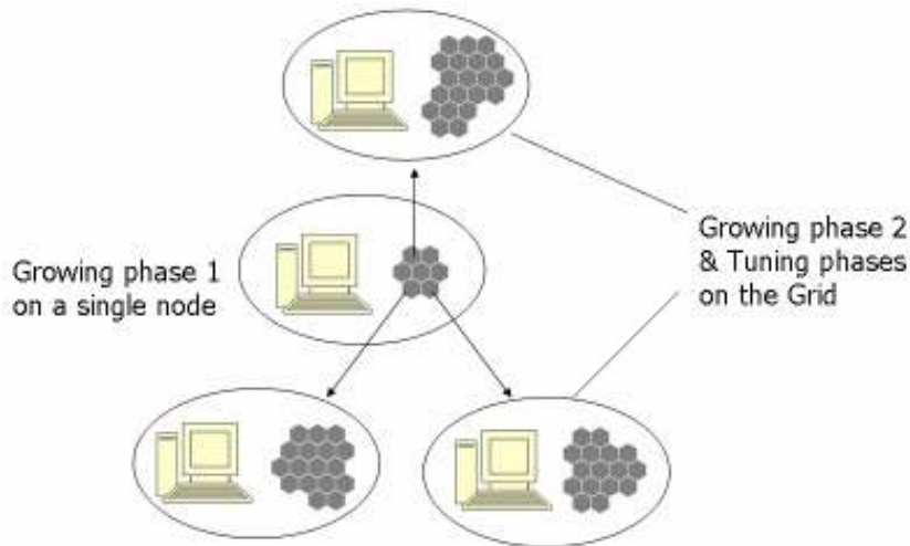
Figure 1. Two stages of scalable GSOM
