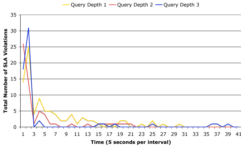
Fig. 4. Total number of SLA violations for bounded H-metric queries.
