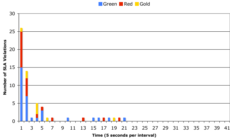
Fig. 5. SLA violations shown by service level for a H-metric query depth of 2.
