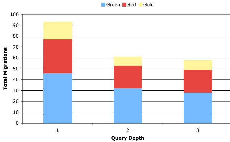
Fig. 6. Total number of violations for each service level for bounded H-metric queries.
