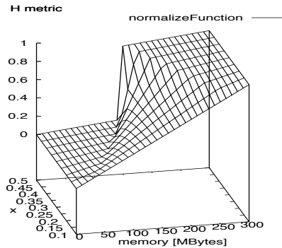
Fig. 3. Normalisation function for memory.
