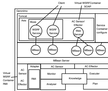
Fig. 1. Internal structure of the WSRF container
