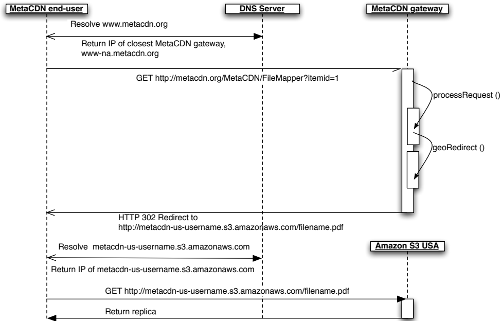
Figure 5. MetaCDN Load Redirector
