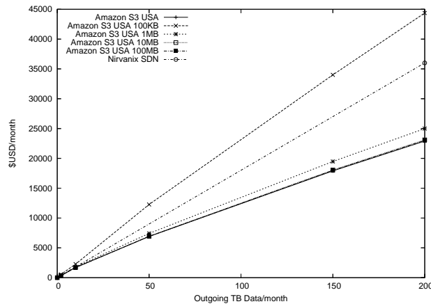
Figure 1. Cloud Storage Pricing
