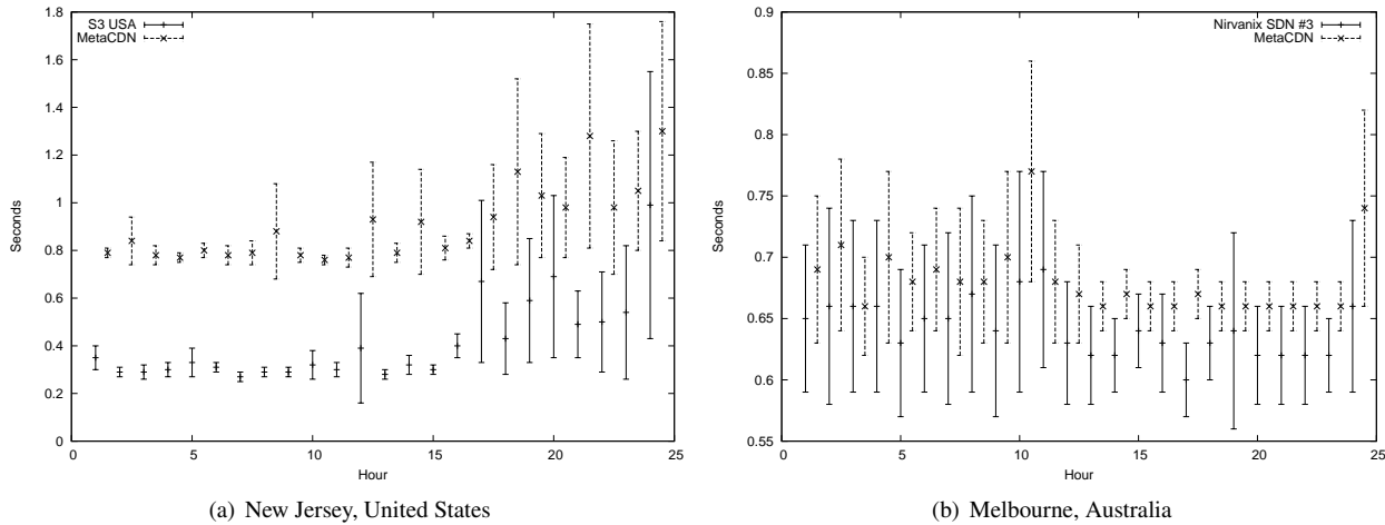
Figure 8. Direct replica access versus MetaCDN Load Redirection
