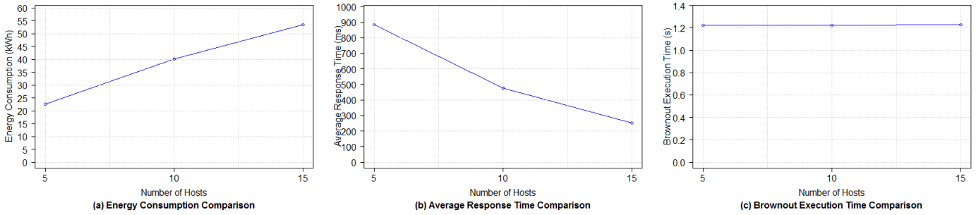
Fig. 9. Scalability Evaluation of iBrownout with LUCF policy
