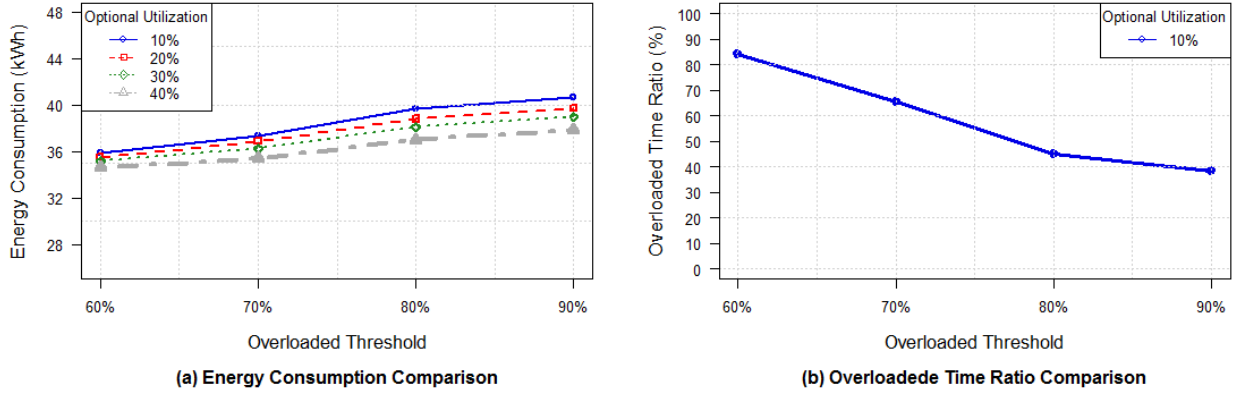
Fig. 5. Algorithm Performance Comparison
