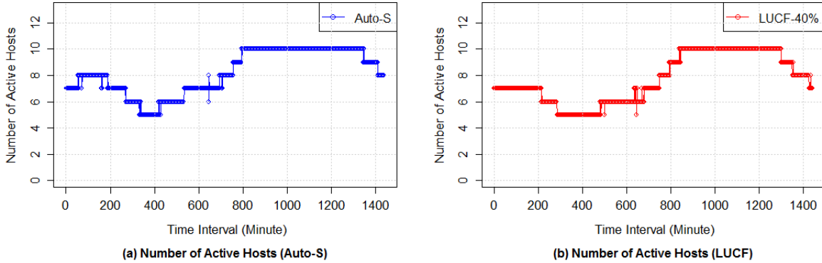
Fig. 8. Number of Active Hosts Comparison
